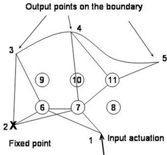
Figure 2: An example design with 6 intermediate connection ports. This design is considered fully connected because pTop_i = 1 for all paths ( i = 1 \sim 7 ).
